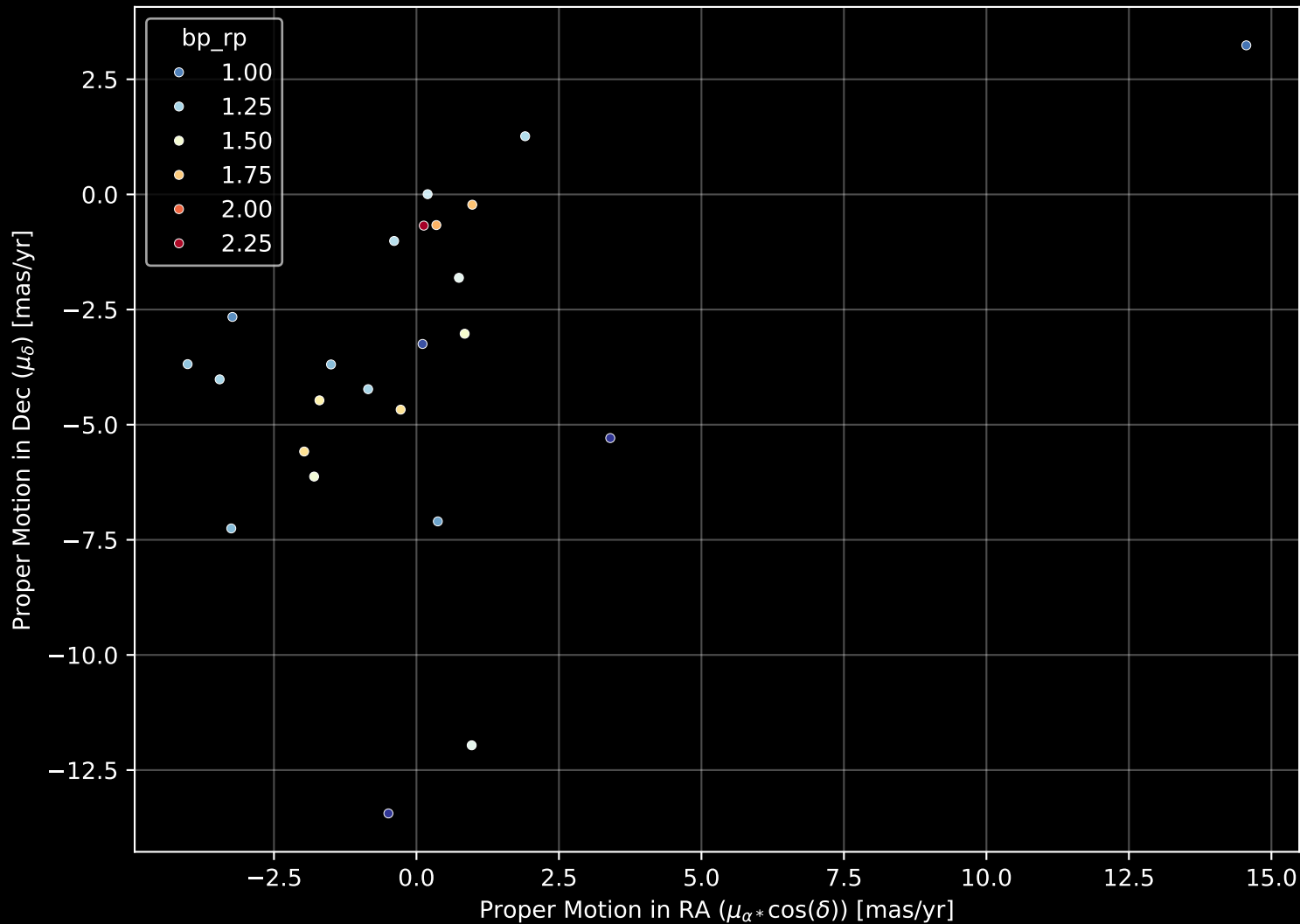
APOGEE DR17 Field: [cepheid] Proper Motion Diagram (n= 24)
